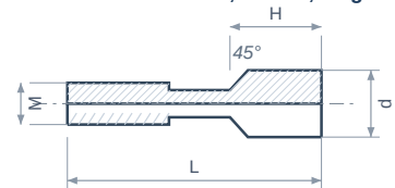
Pull stud — thread M, head d, length L
